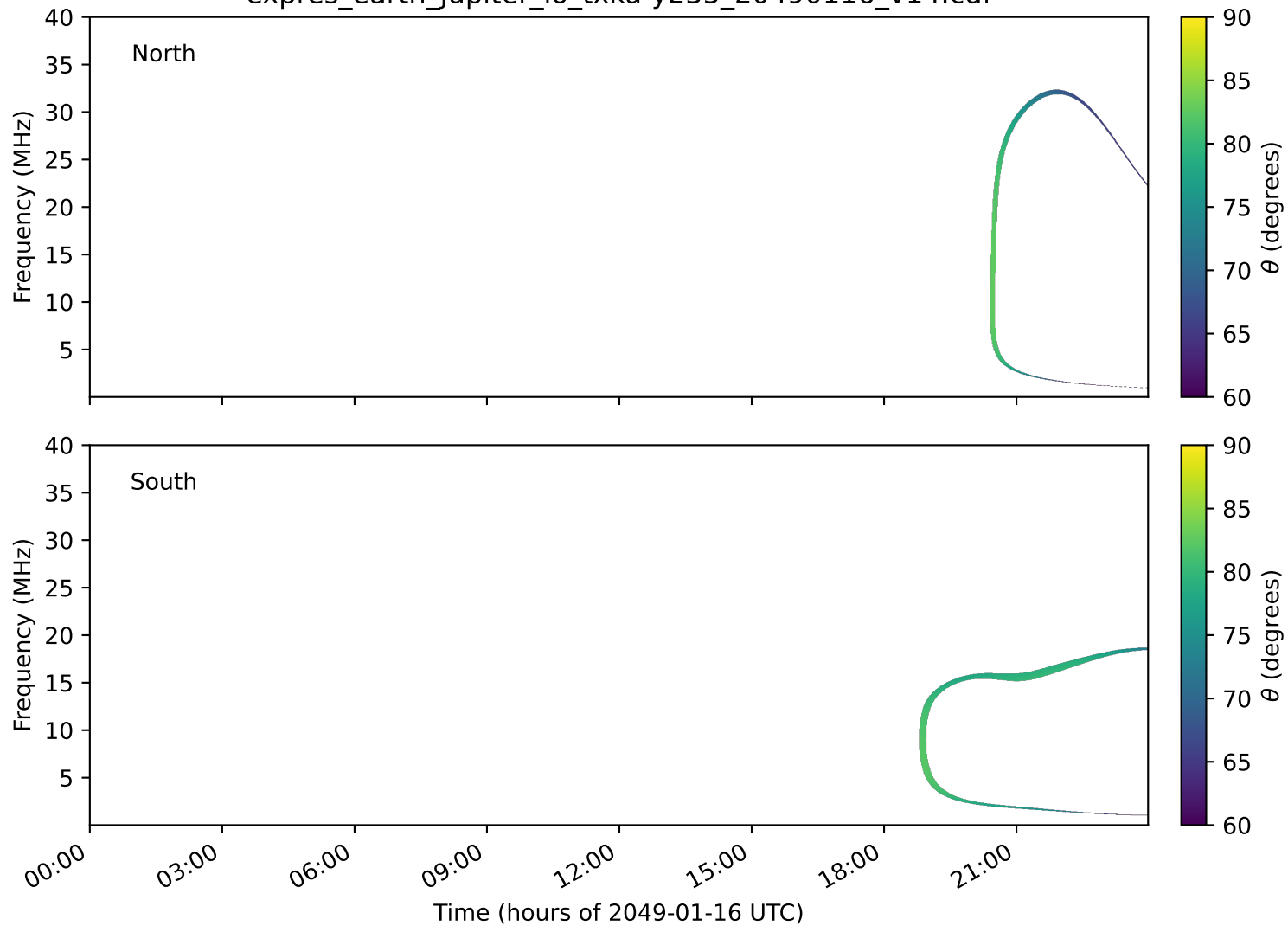
expres_earth_jupiter_io_txka-y235_20490116_v14.cdf
