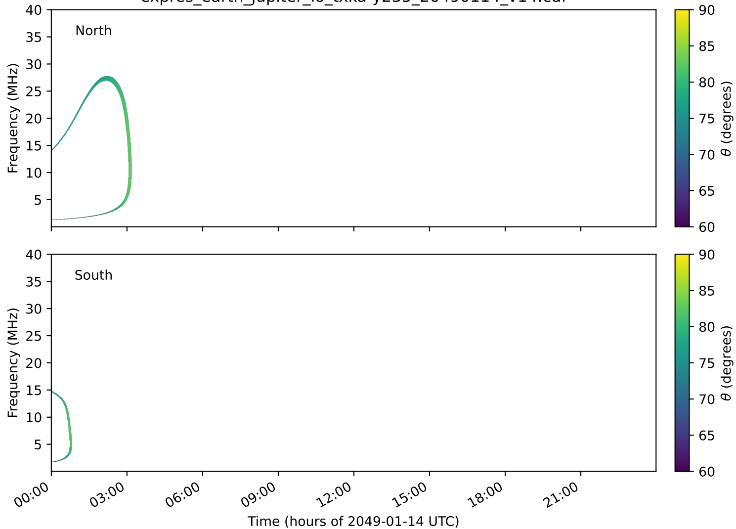
expres_earth_jupiter_io_txka-y235_20490114_v14.cdf
