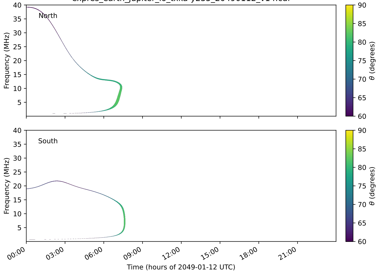
expres_earth_jupiter_io_txka-y235_20490112_v14.cdf
