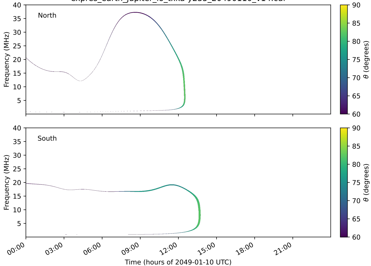
expres_earth_jupiter_io_txka-y235_20490110_v14.cdf
