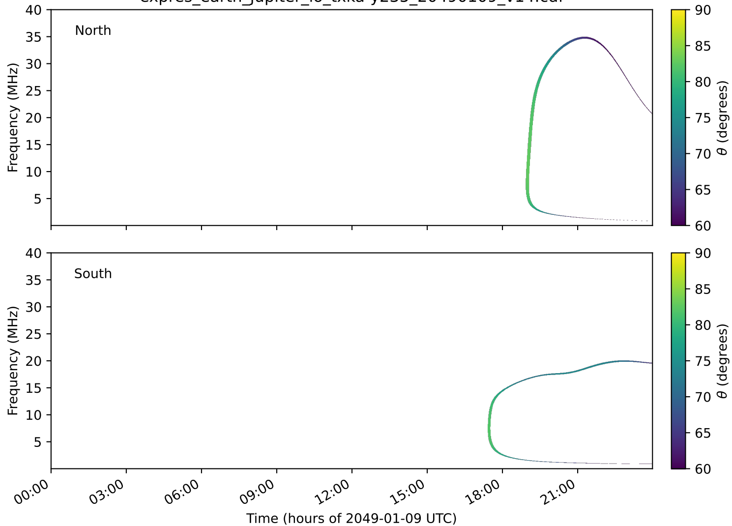
expres_earth_jupiter_io_txka-y235_20490109_v14.cdf
