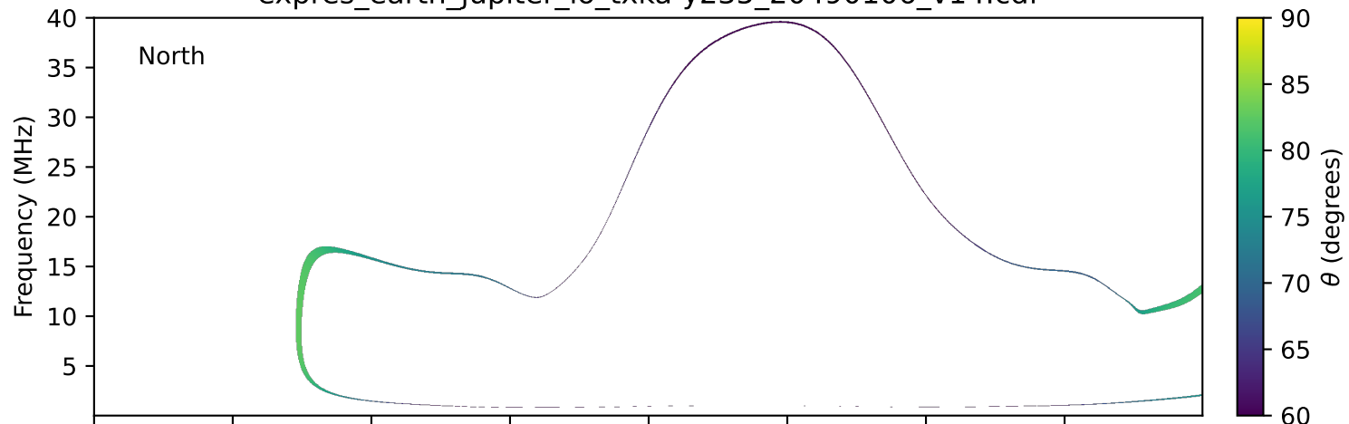
expres_earth_jupiter_io_txka-y235_20490106_v14.cdf
