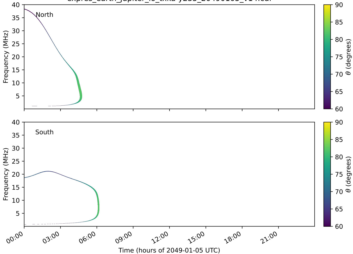
expres_earth_jupiter_io_txka-y235_20490105_v14.cdf
