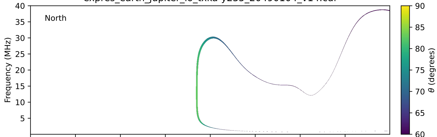
expres_earth_jupiter_io_txka-y235_20490104_v14.cdf
