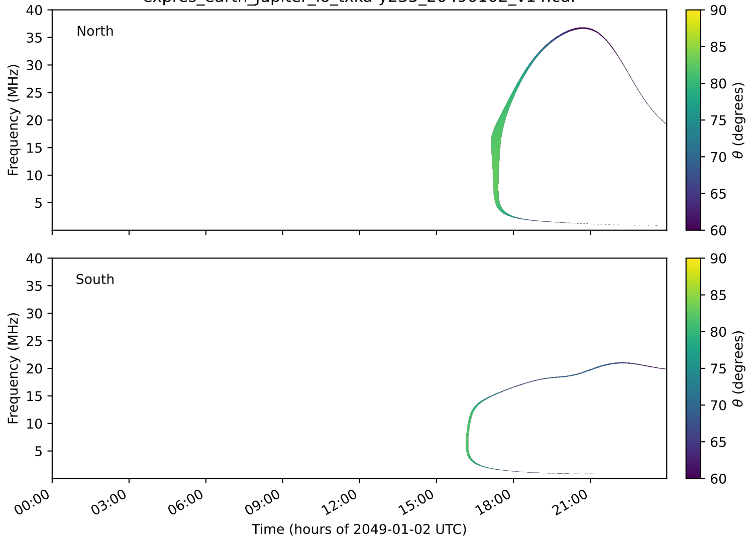
expres_earth_jupiter_io_txka-y235_20490102_v14.cdf
