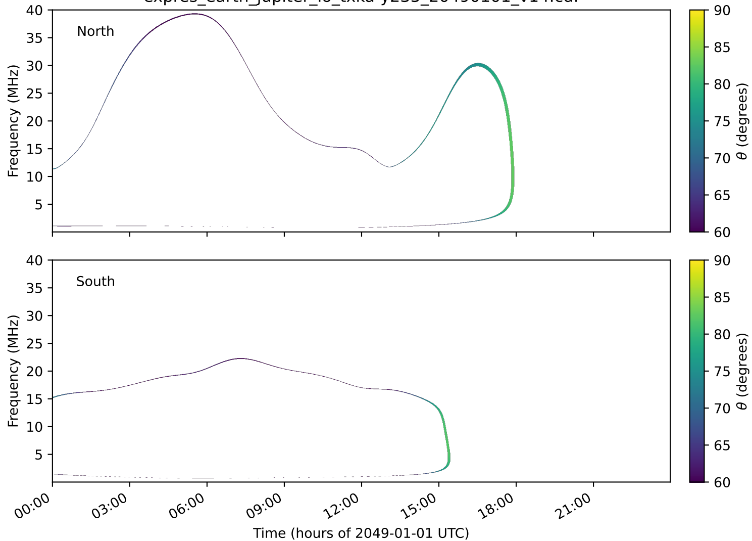
expres_earth_jupiter_io_txka-y235_20490101_v14.cdf
