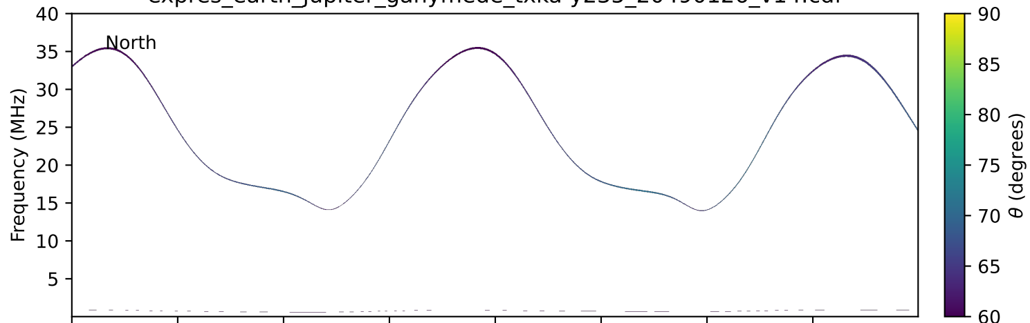
expres_earth_jupiter_ganymede_txka-y235_20490126_v14.cdf
