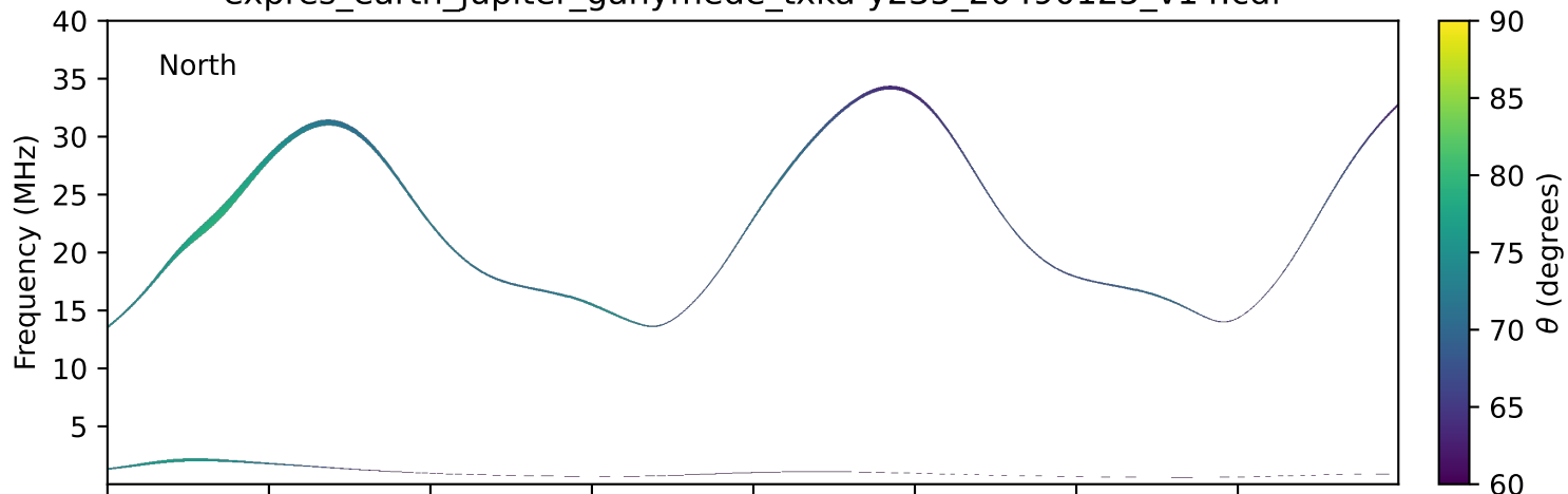
expres_earth_jupiter_ganymede_txka-y235_20490125_v14.cdf
