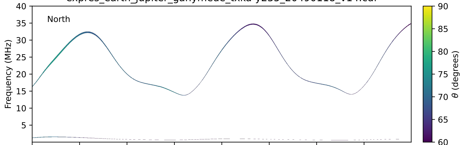
expres_earth_jupiter_ganymede_txka-y235_20490118_v14.cdf
