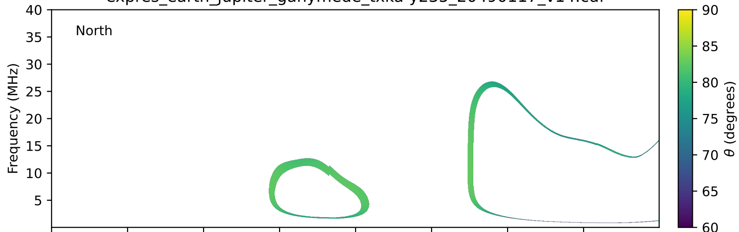
expres_earth_jupiter_ganymede_txka-y235_20490117_v14.cdf
