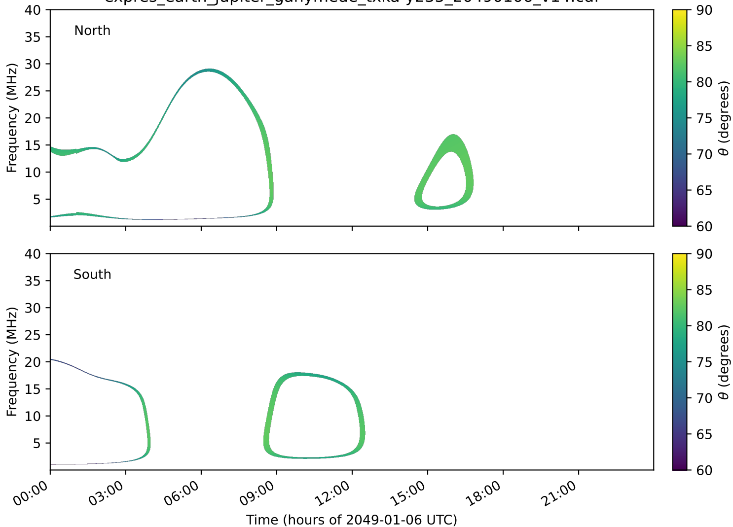
expres_earth_jupiter_ganymede_txka-y235_20490106_v14.cdf
