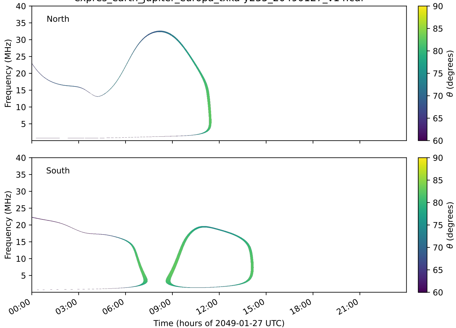
expres_earth_jupiter_europa_txka-y235_20490127_v14.cdf
