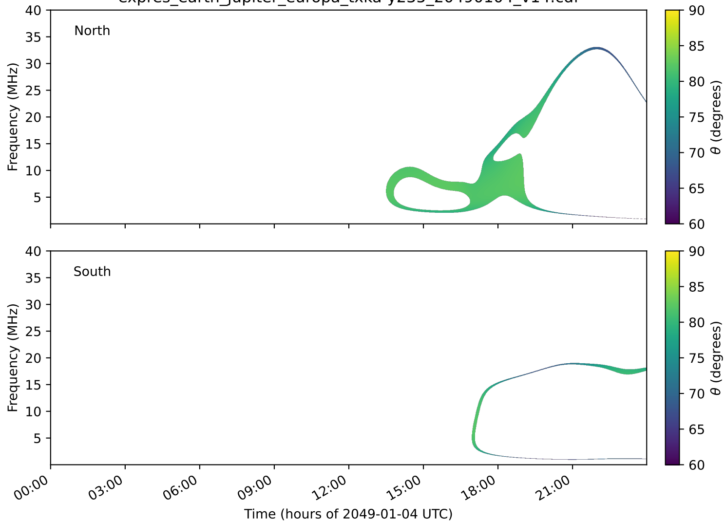
expres_earth_jupiter_europa_txka-y235_20490104_v14.cdf
