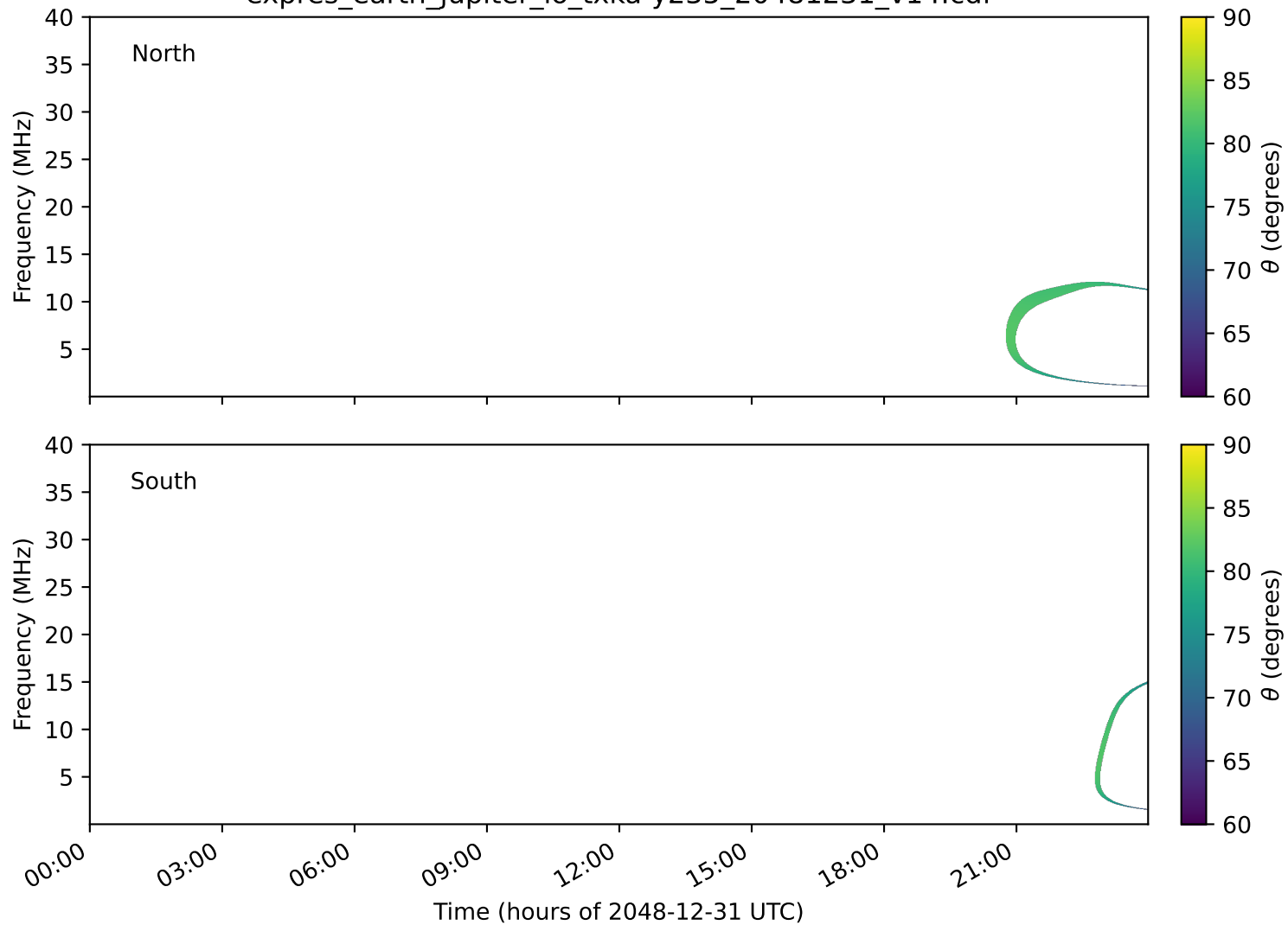
expres_earth_jupiter_io_txka-y235_20481231_v14.cdf
