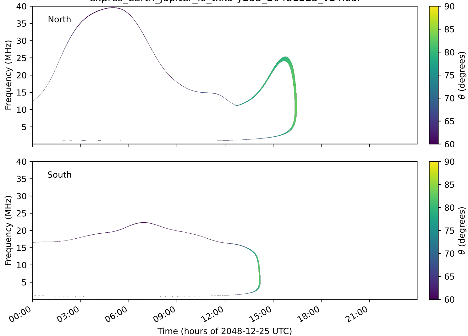
expres_earth_jupiter_io_txka-y235_20481225_v14.cdf
