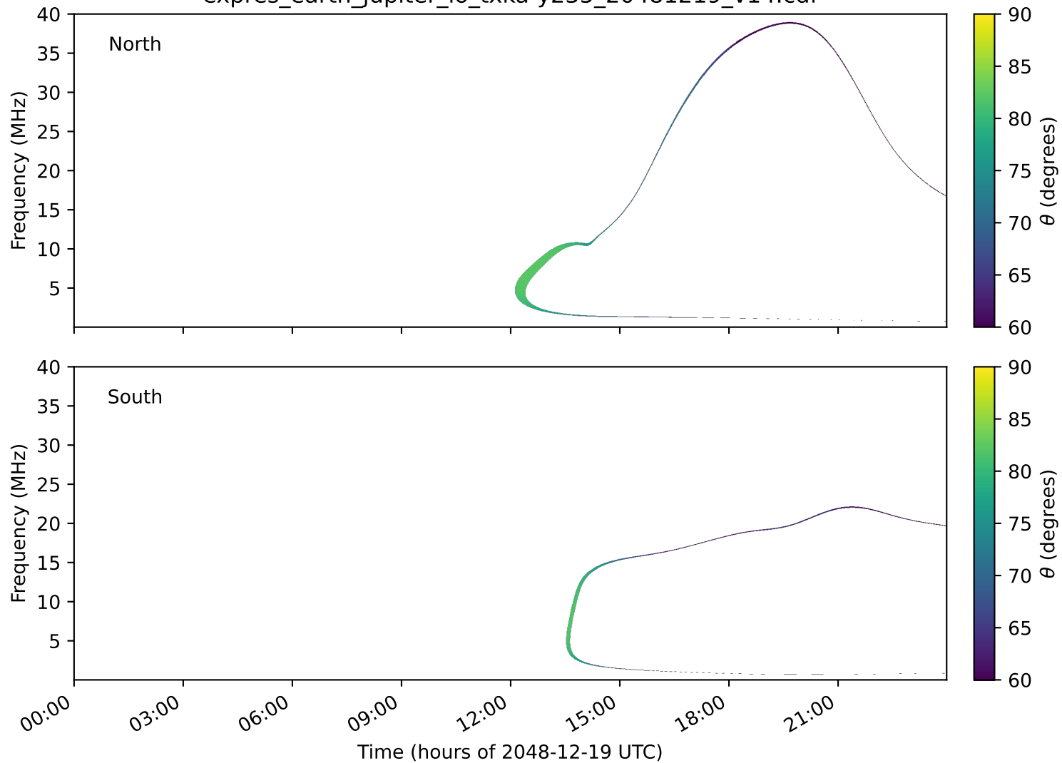
expres_earth_jupiter_io_txka-y235_20481219_v14.cdf
