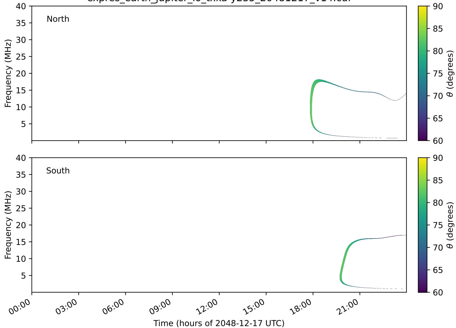
expres_earth_jupiter_io_txka-y235_20481217_v14.cdf
