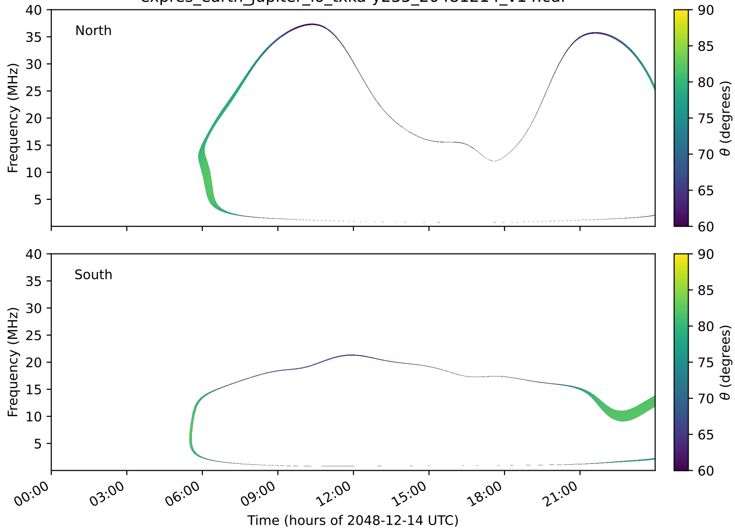
expres_earth_jupiter_io_txka-y235_20481214_v14.cdf
