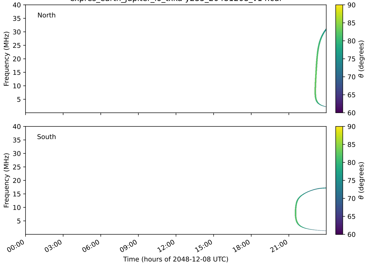
expres_earth_jupiter_io_txka-y235_20481208_v14.cdf
