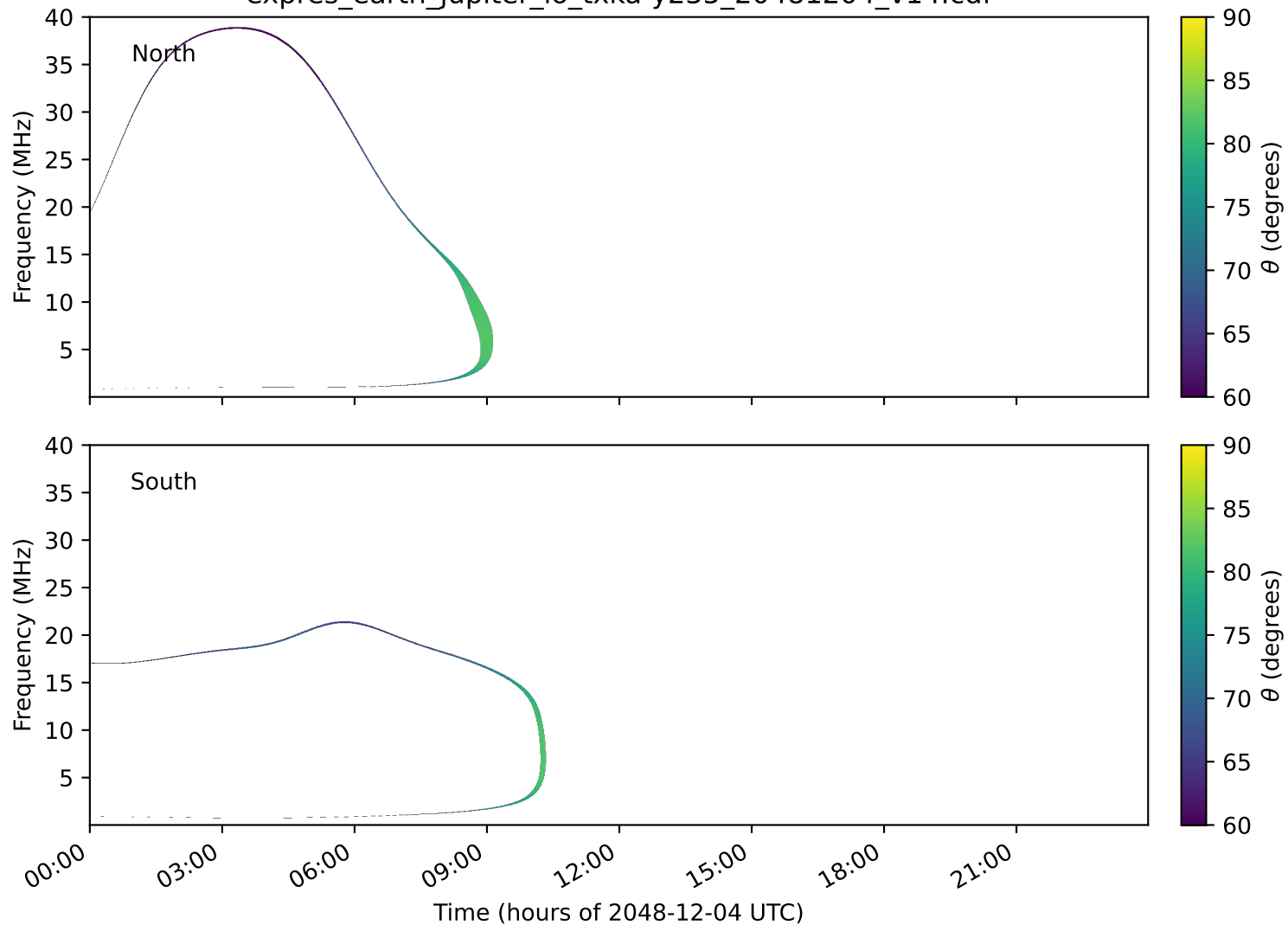
expres_earth_jupiter_io_txka-y235_20481204_v14.cdf
