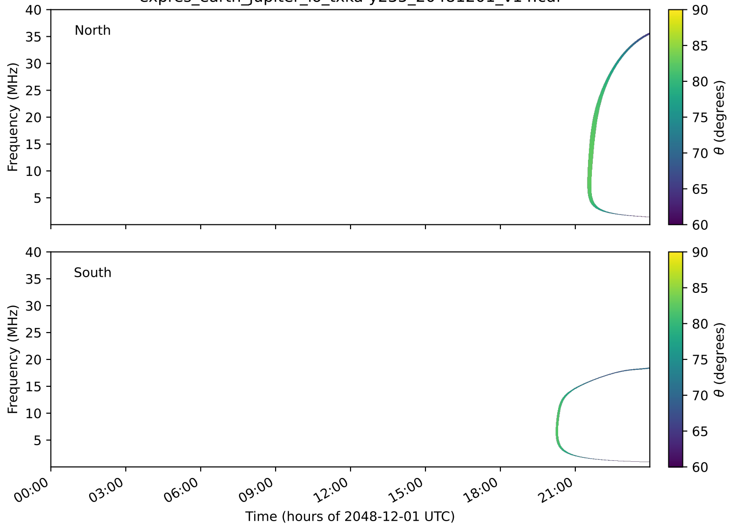
expres_earth_jupiter_io_txka-y235_20481201_v14.cdf
