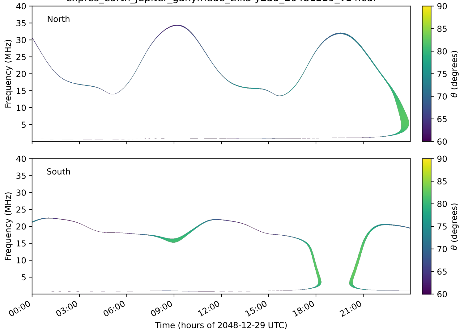
expres_earth_jupiter_ganymede_txka-y235_20481229_v14.cdf
