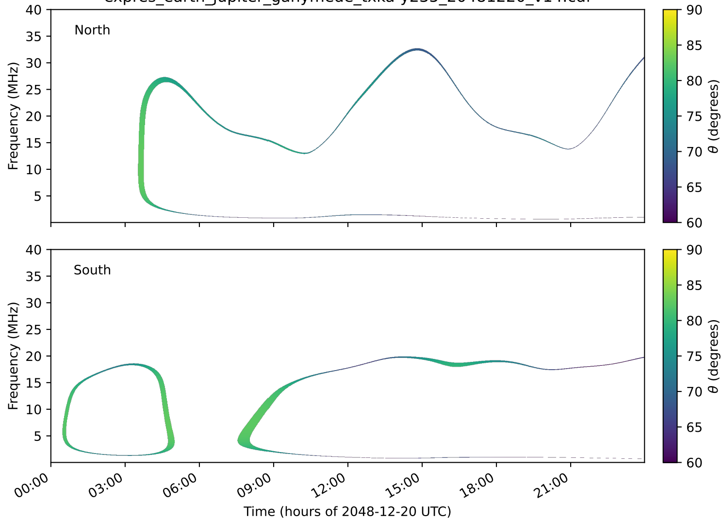
expres_earth_jupiter_ganymede_txka-y235_20481220_v14.cdf
