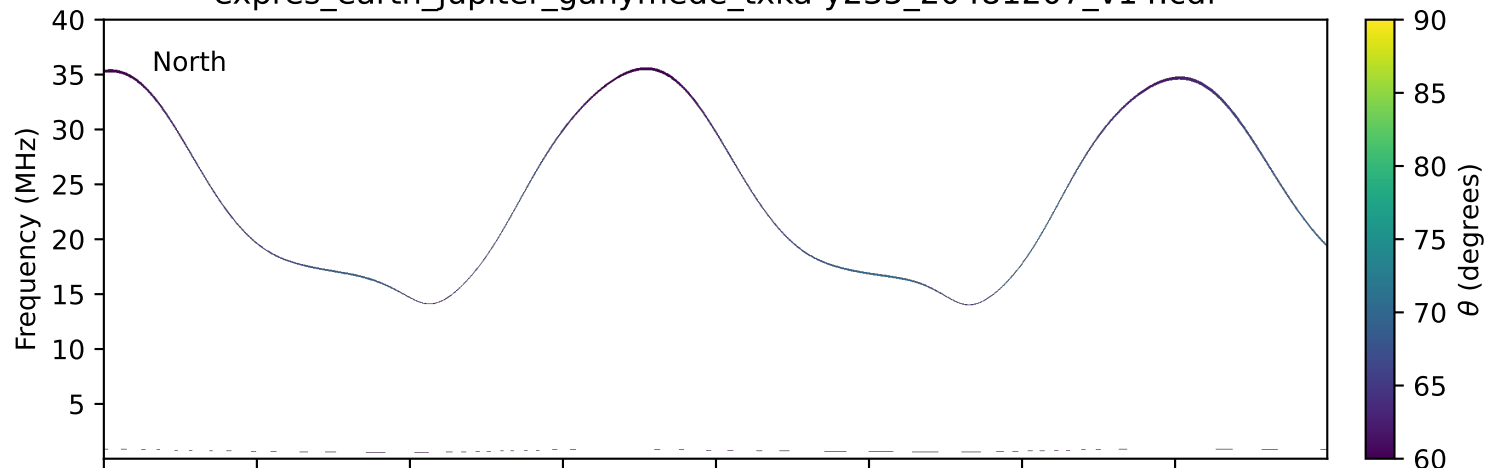
expres_earth_jupiter_ganymede_txka-y235_20481207_v14.cdf
