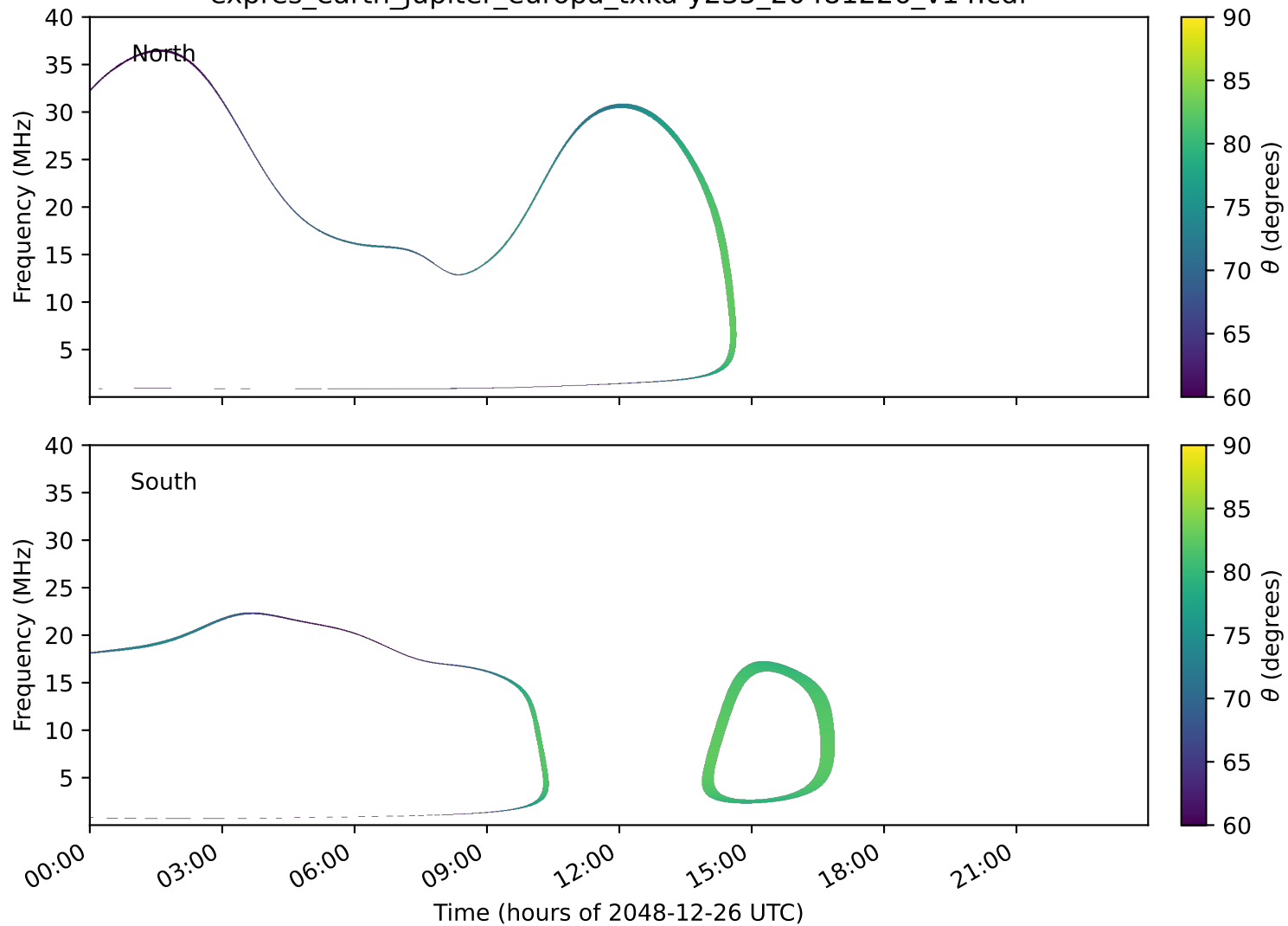
expres_earth_jupiter_europa_txka-y235_20481226_v14.cdf
