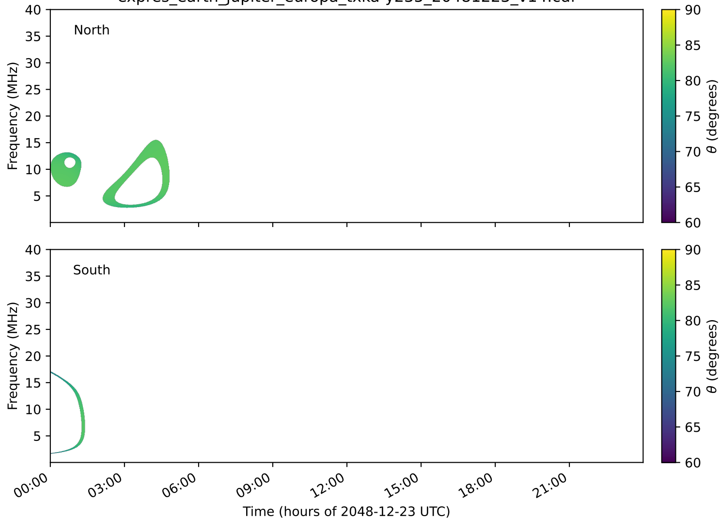
expres_earth_jupiter_europa_txka-y235_20481223_v14.cdf
