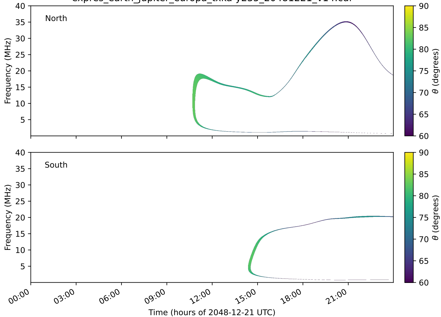
expres_earth_jupiter_europa_txka-y235_20481221_v14.cdf
