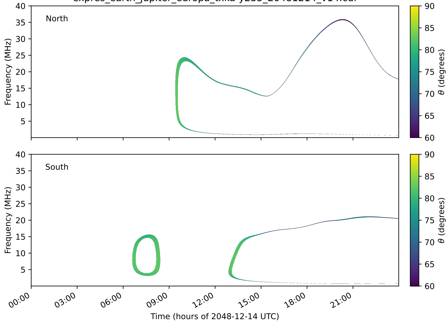
expres_earth_jupiter_europa_txka-y235_20481214_v14.cdf
