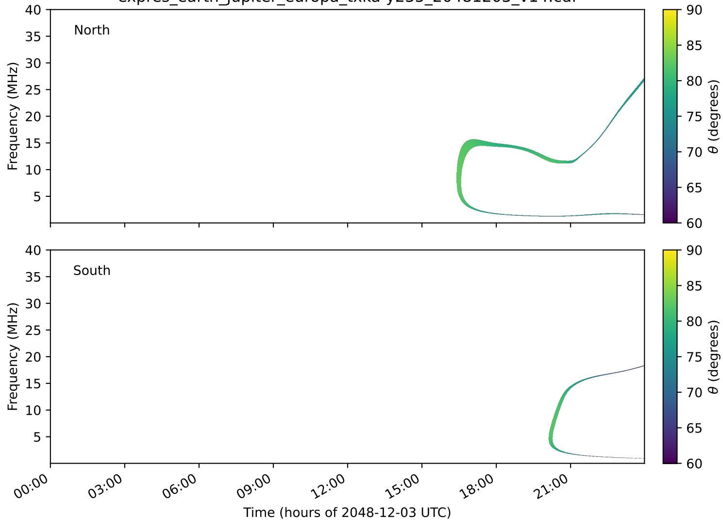
expres_earth_jupiter_europa_txka-y235_20481203_v14.cdf
