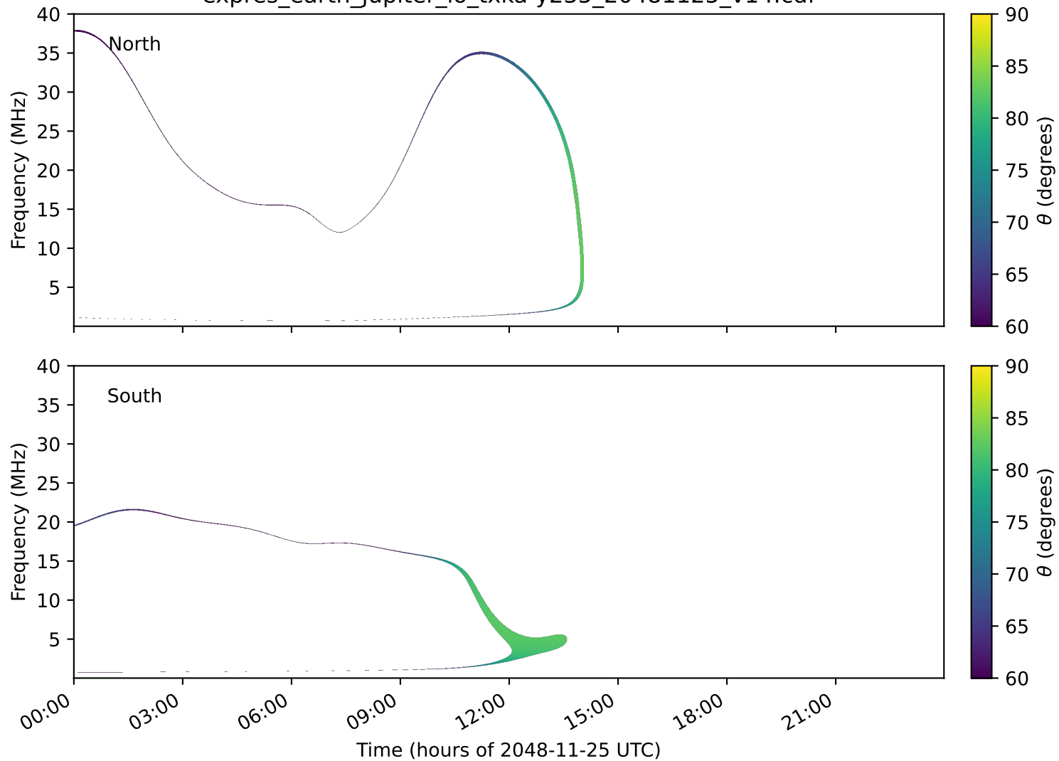
expres_earth_jupiter_io_txka-y235_20481125_v14.cdf
