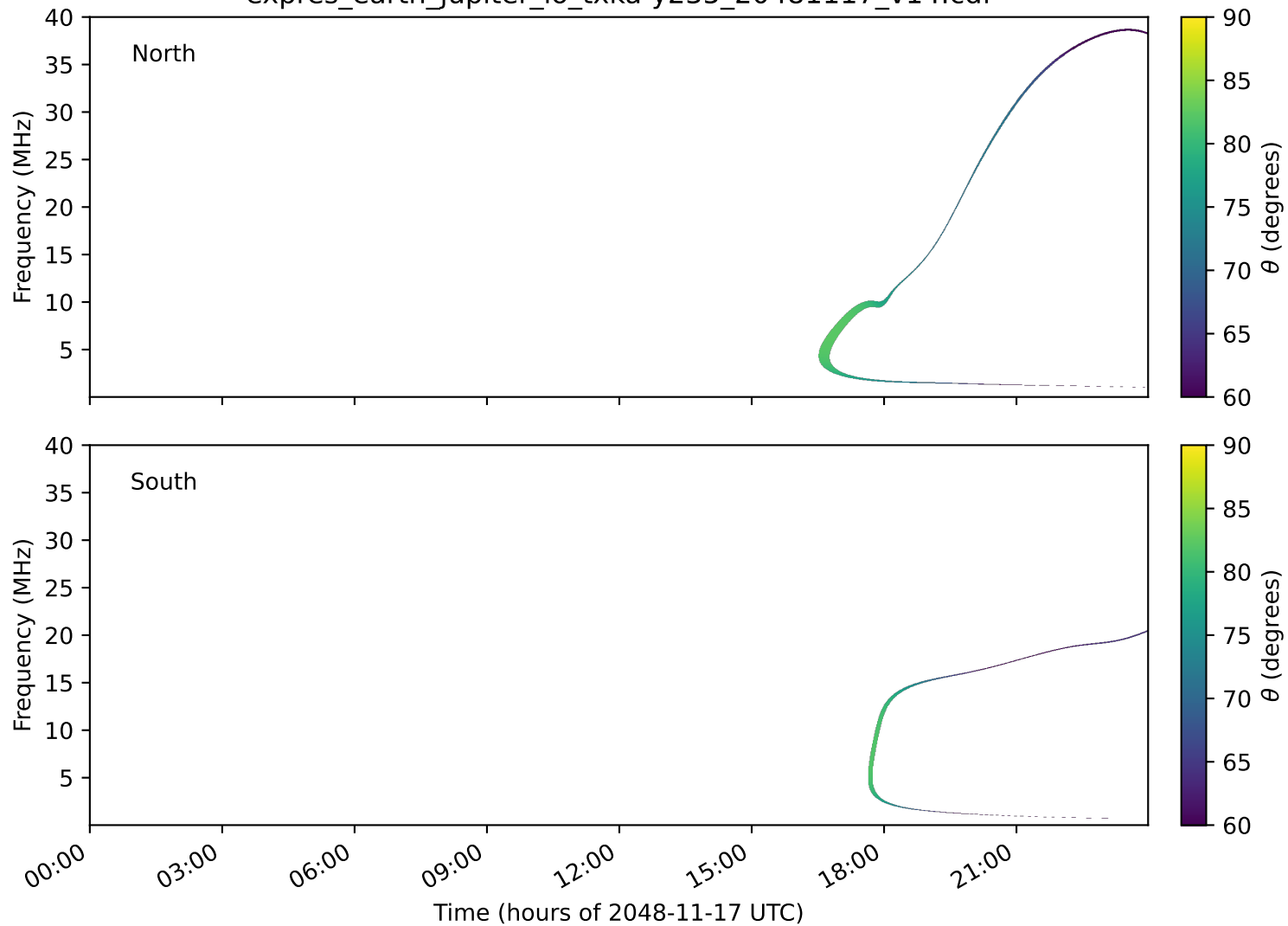
expres_earth_jupiter_io_txka-y235_20481117_v14.cdf
