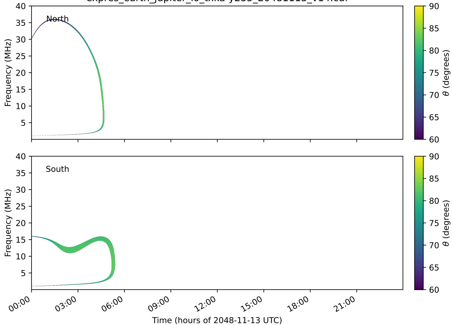
expres_earth_jupiter_io_txka-y235_20481113_v14.cdf
