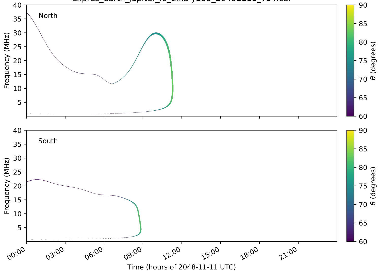
expres_earth_jupiter_io_txka-y235_20481111_v14.cdf
