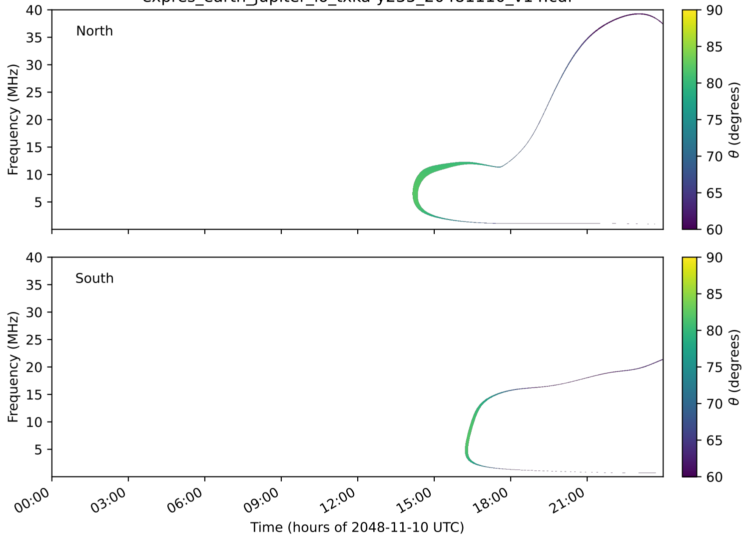
expres_earth_jupiter_io_txka-y235_20481110_v14.cdf
