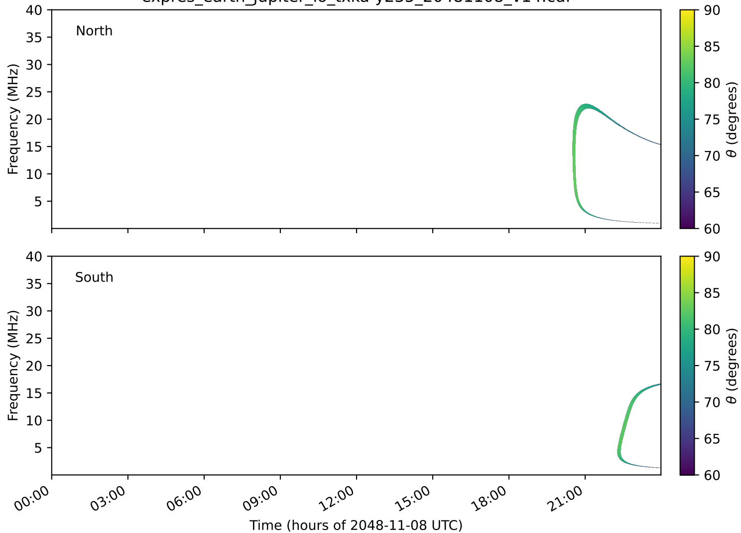
expres_earth_jupiter_io_txka-y235_20481108_v14.cdf
