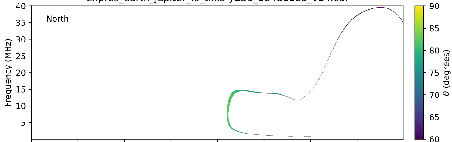
expres_earth_jupiter_io_txka-y235_20481103_v14.cdf
