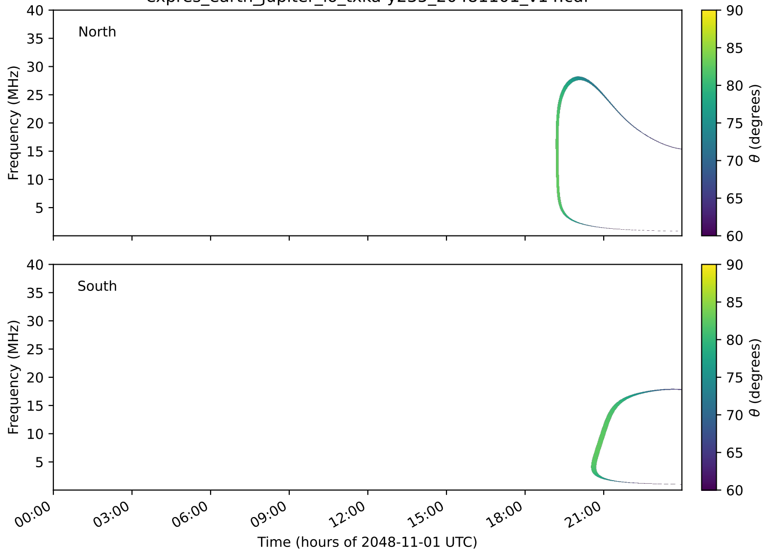
expres_earth_jupiter_io_txka-y235_20481101_v14.cdf
