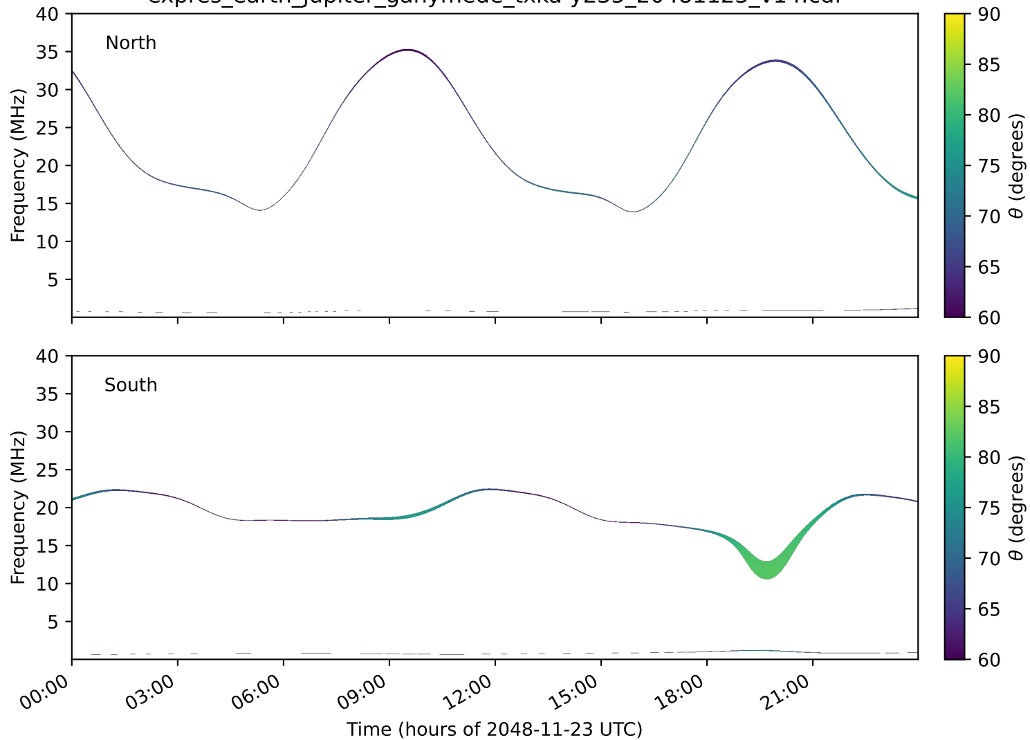
expres_earth_jupiter_ganymede_txka-y235_20481123_v14.cdf
