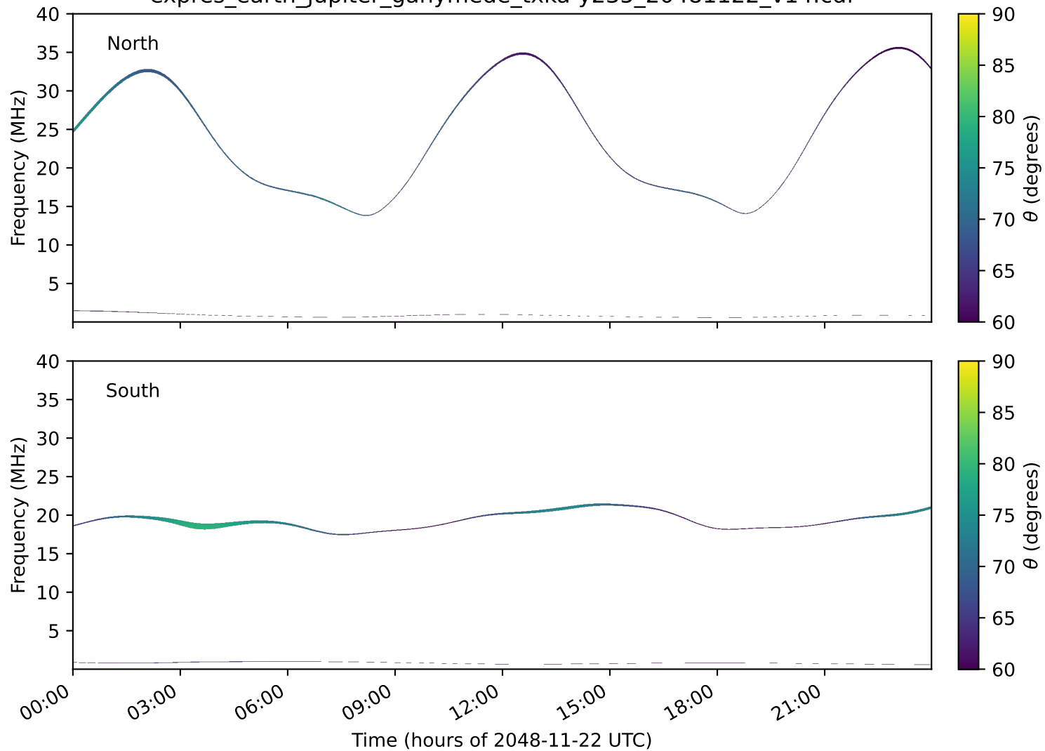
expres_earth_jupiter_ganymede_txka-y235_20481122_v14.cdf
