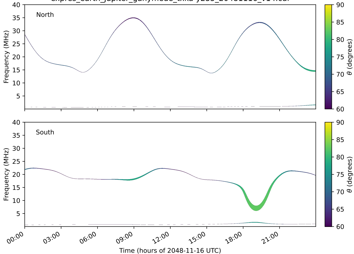
expres_earth_jupiter_ganymede_txka-y235_20481116_v14.cdf
