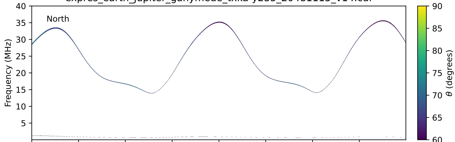
expres_earth_jupiter_ganymede_txka-y235_20481115_v14.cdf
