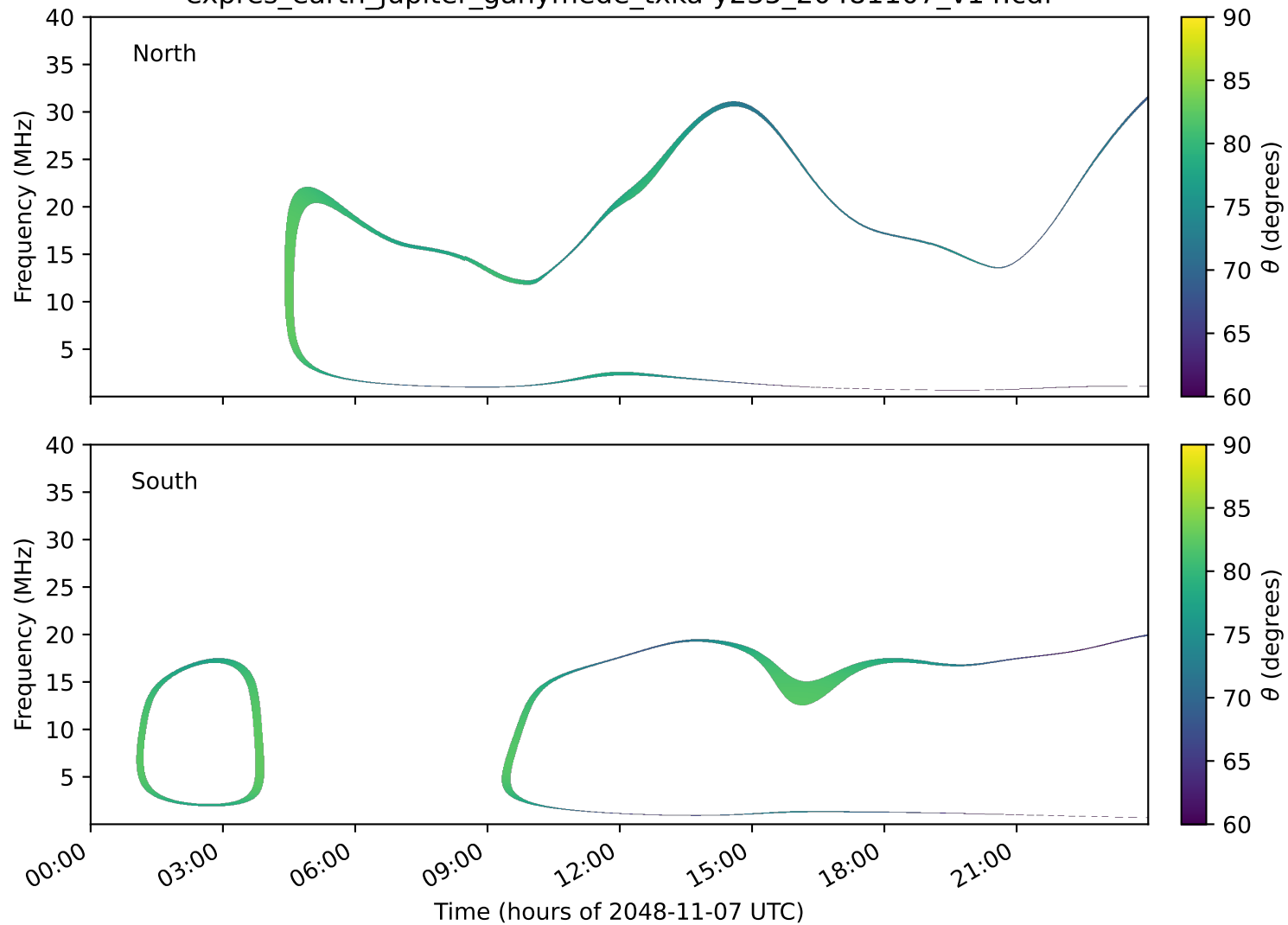
expres_earth_jupiter_ganymede_txka-y235_20481107_v14.cdf
