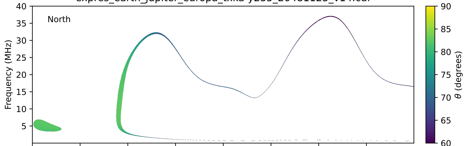
expres_earth_jupiter_europa_txka-y235_20481123_v14.cdf
