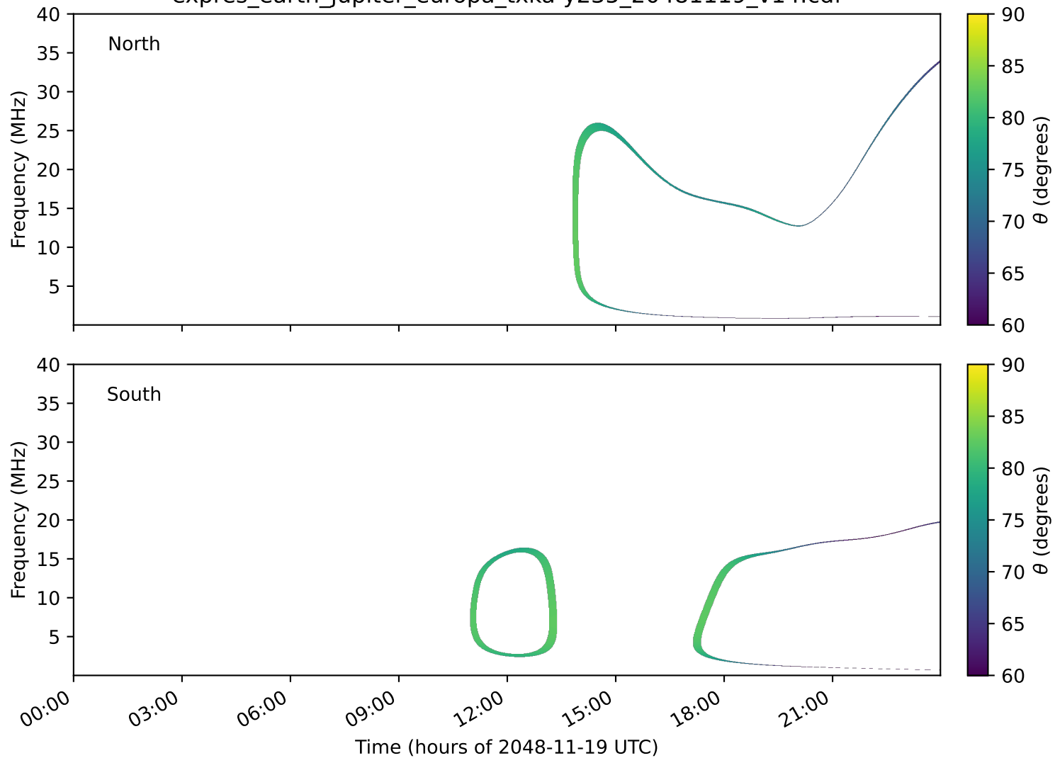
expres_earth_jupiter_europa_txka-y235_20481119_v14.cdf
