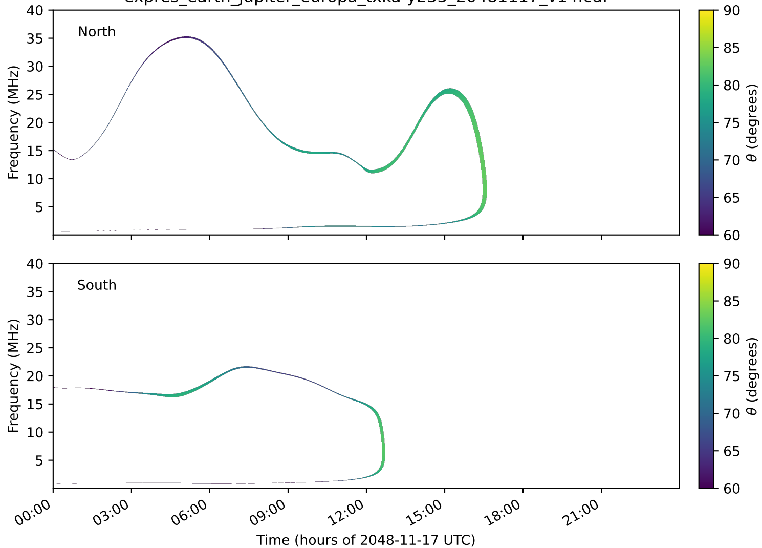
expres_earth_jupiter_europa_txka-y235_20481117_v14.cdf
