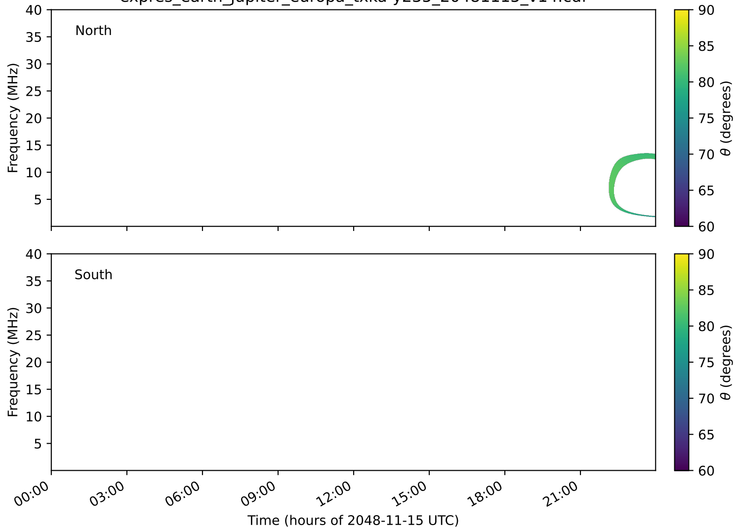
expres_earth_jupiter_europa_txka-y235_20481115_v14.cdf
